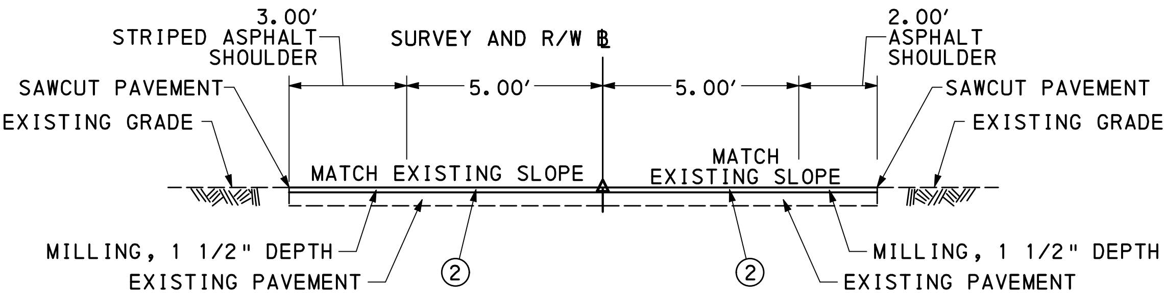
OHIO RIVER TRAIL PHASE 1 - TYPICAL SECTION STA 223+97.00 TO STA 224+87.00 STA 226+91.00 TO 227+67.55 NOT TO SCALE
