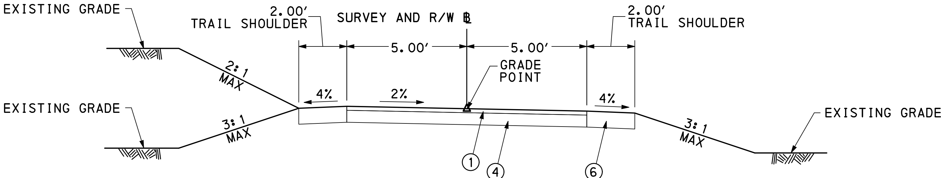
OHIO RIVER TRAIL PHASE 1 - TYPICAL SECTION STA 205+50.00 TO STA 209+03.21 STA 209+42.30 TO 223+97.00 NOT TO SCALE
