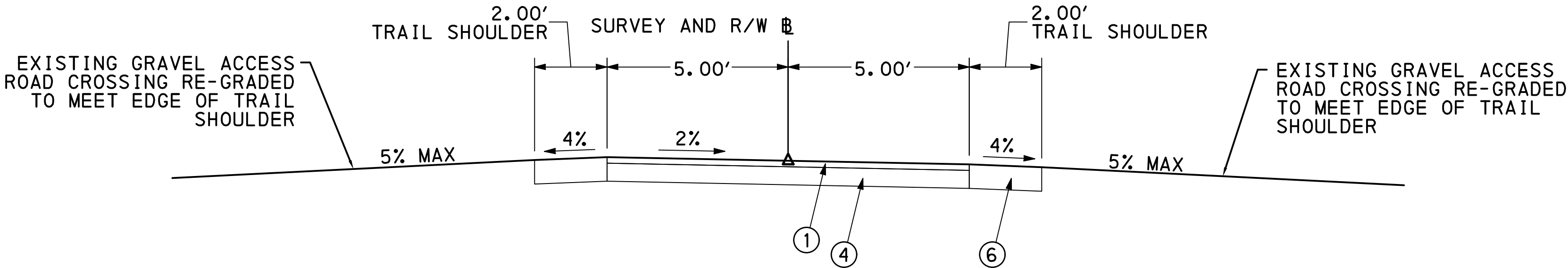
OHIO RIVER TRAIL PHASE 1 - TYPICAL SECTION STA 205+35.00 TO STA 205+50.00 NOT TO SCALE
