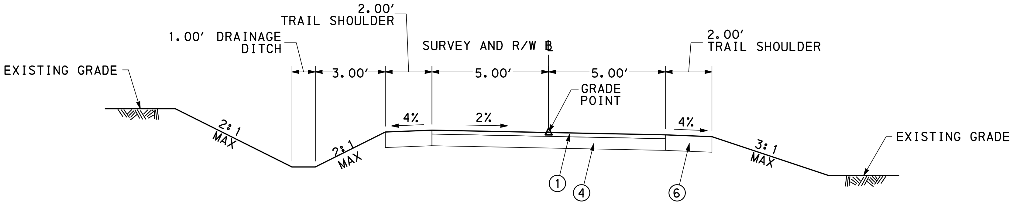
OHIO RIVER TRAIL PHASE 1 - TYPICAL SECTION STA 200+20.00 TO STA 205+35.00 NOT TO SCALE
