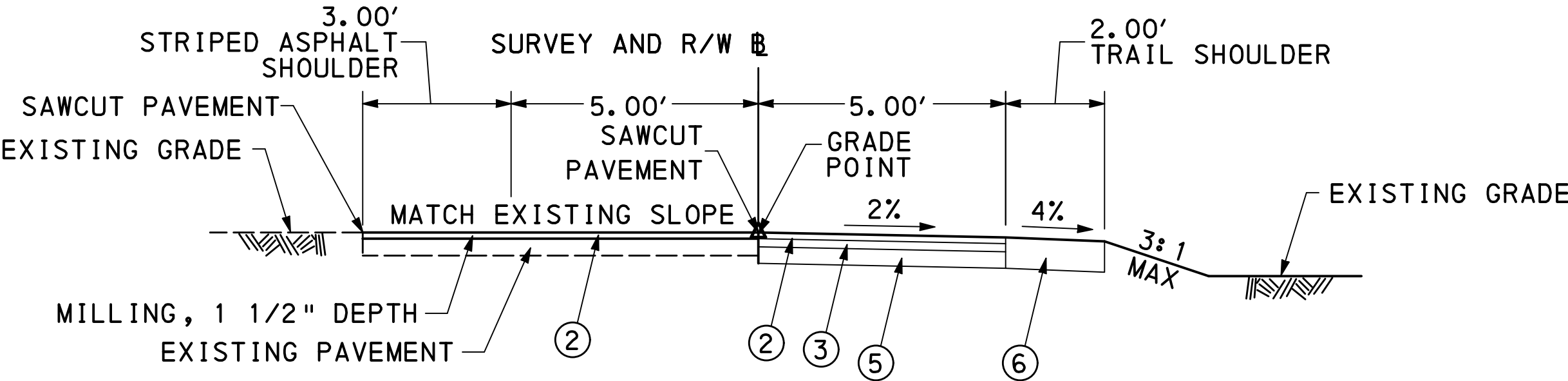
OHIO RIVER TRAIL PHASE 1 - TYPICAL SECTION STA 224+87.00 TO STA 226+91.00 NOT TO SCALE
